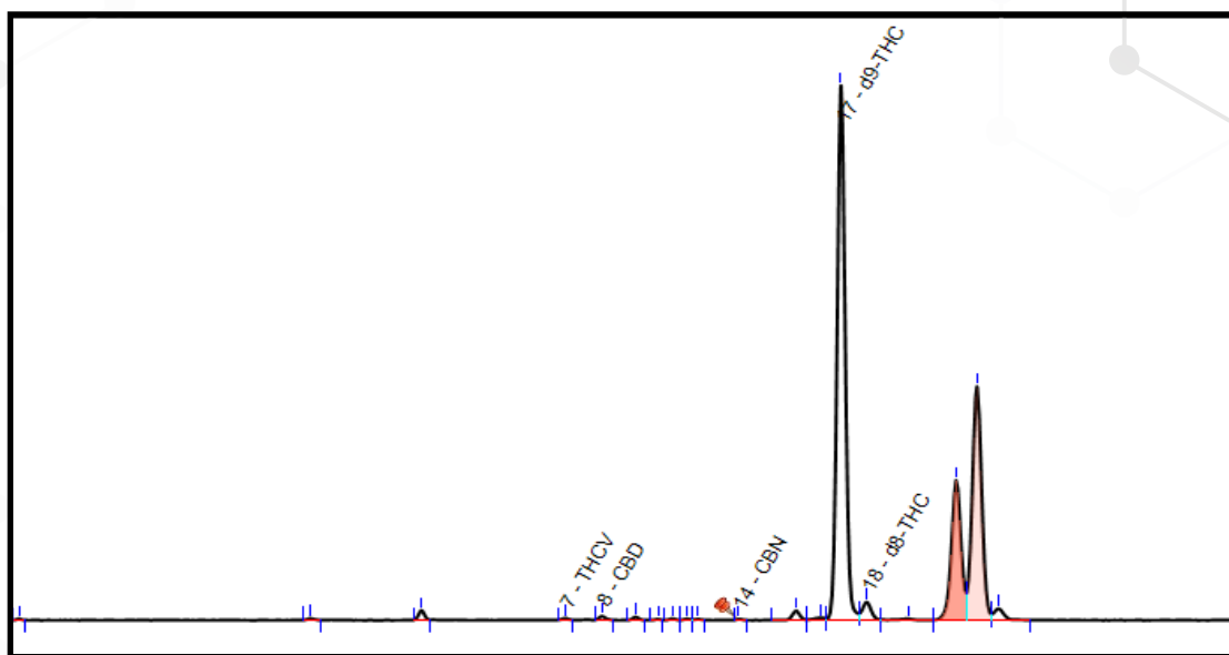
Figure 1. UHPLC-PDA chromatogram of Pure Relief Party Time Strawnana
