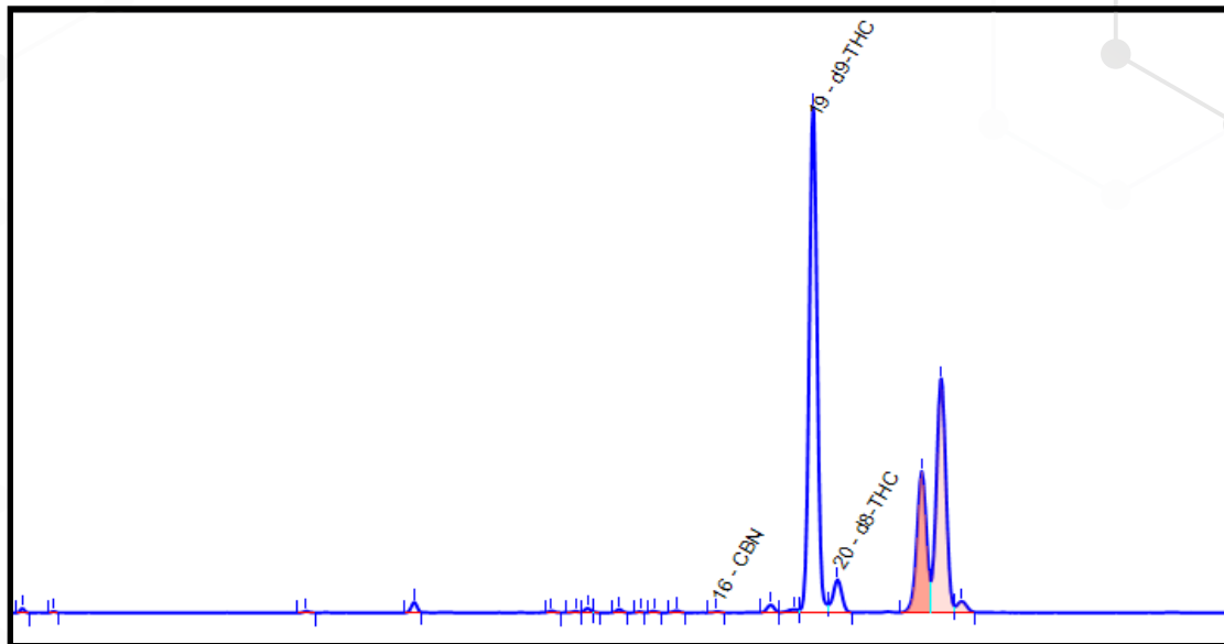
Figure 1. UHPLC-PDA chromatogram of Pure Relief Party Time Strawberry Cream D9 + HHC
