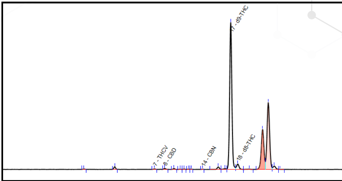
Figure 1. UHPLC-PDA chromatogram of Pure Relief Party Time Pineapple
