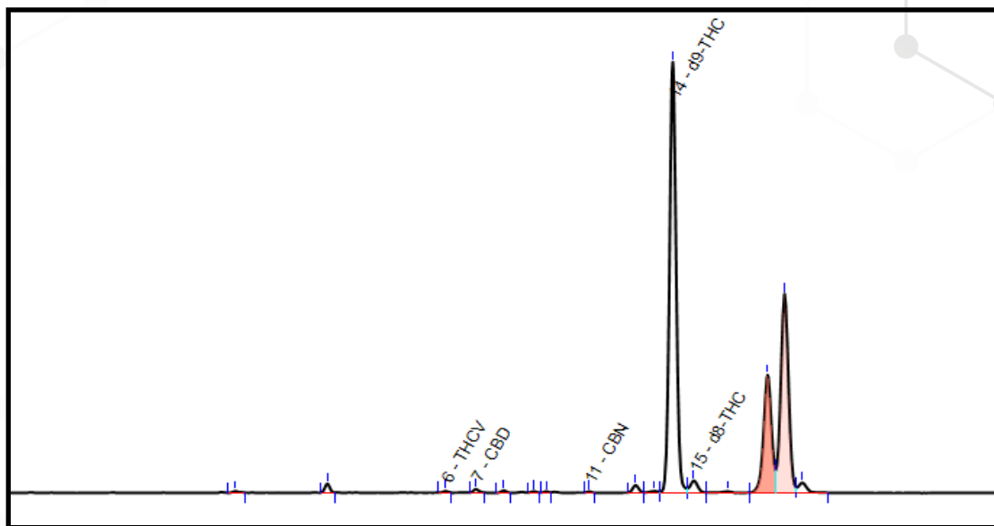
Figure 1. UHPLC-PDA chromatogram of Pure Relief Party Time Acai
